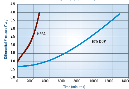
HEPA VS. 95% DOP***
